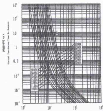
690V 时间电流特性曲线 Time-Current Curve
